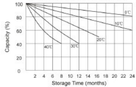
Self-discharge characteristic
